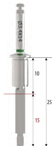
Pilot Drill 25mm(15mm)
