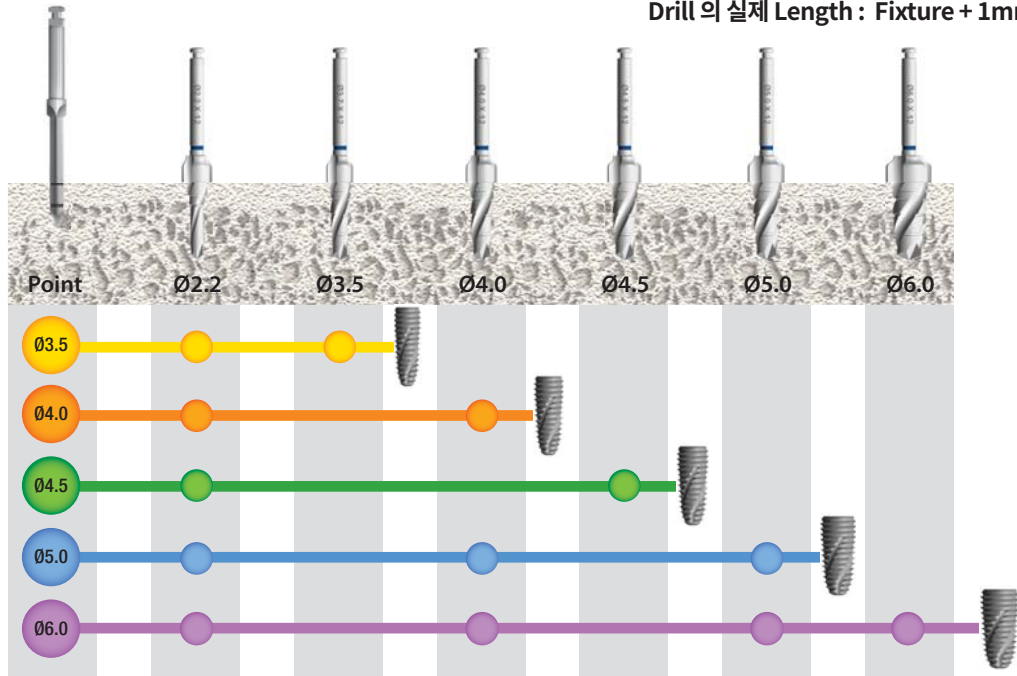
Ø2.2 Initial Drill과 Final Drill를 이용한 간단한 Drill sequence (Ø3.5 / 4.0 / 4.5 fixture)
